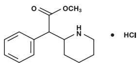
Methylphenidate Hydrochloride C_{14}H_{19}NO_2 \cdot HCl MW = 269.77
